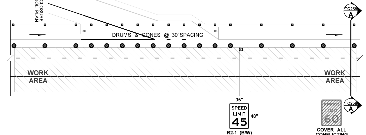
CLOSED LEFT ON-RAMP DETAIL
