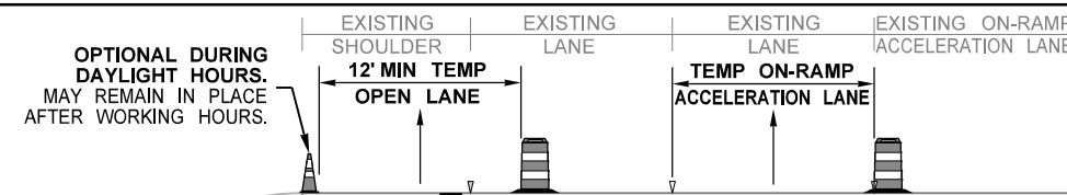
SECTION B-B
