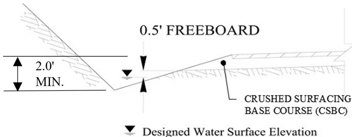
Figure 4-7 Drainage Ditch Detail
