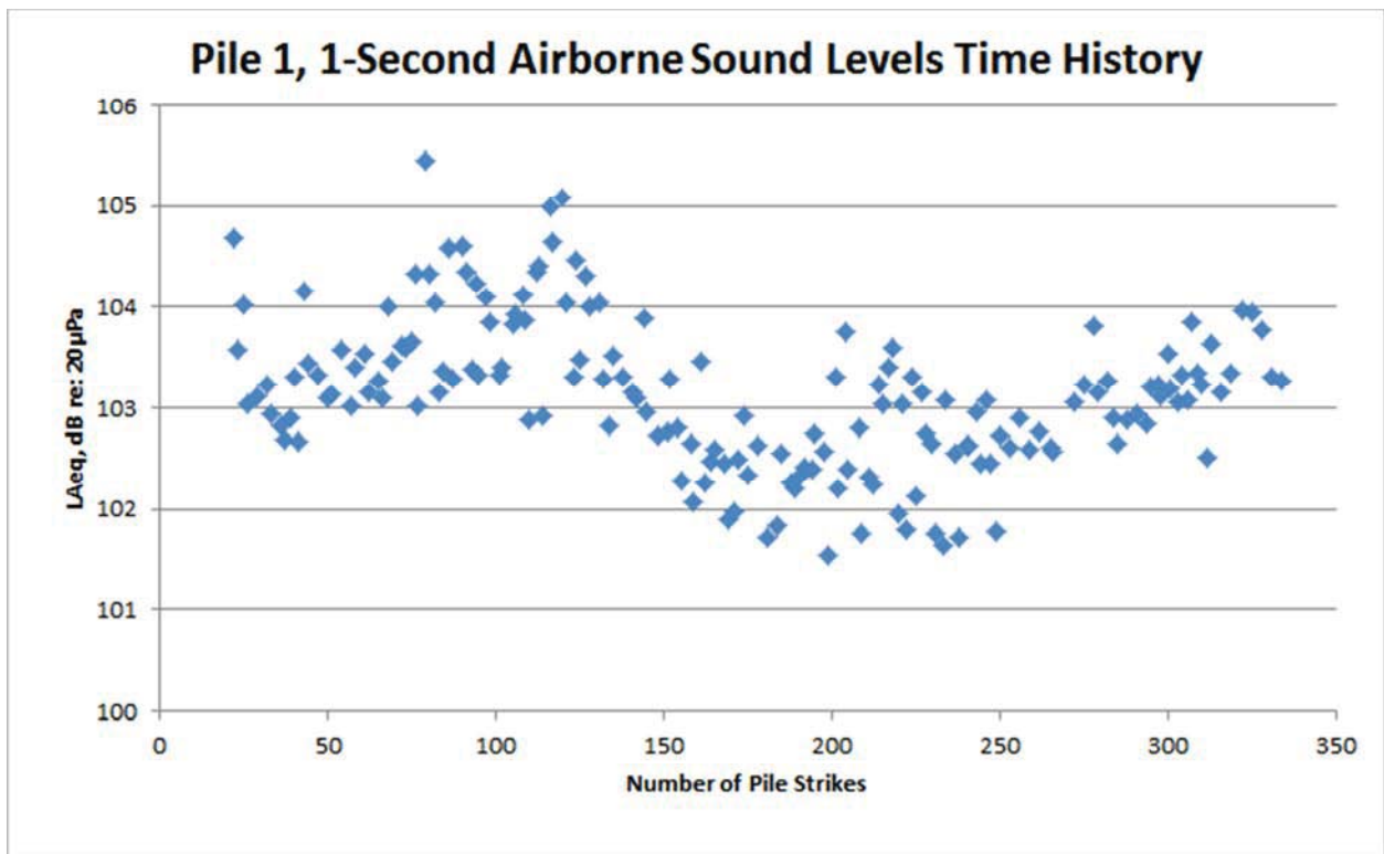
Figure 74: Pile 1, east of Foster Island airborne time history
