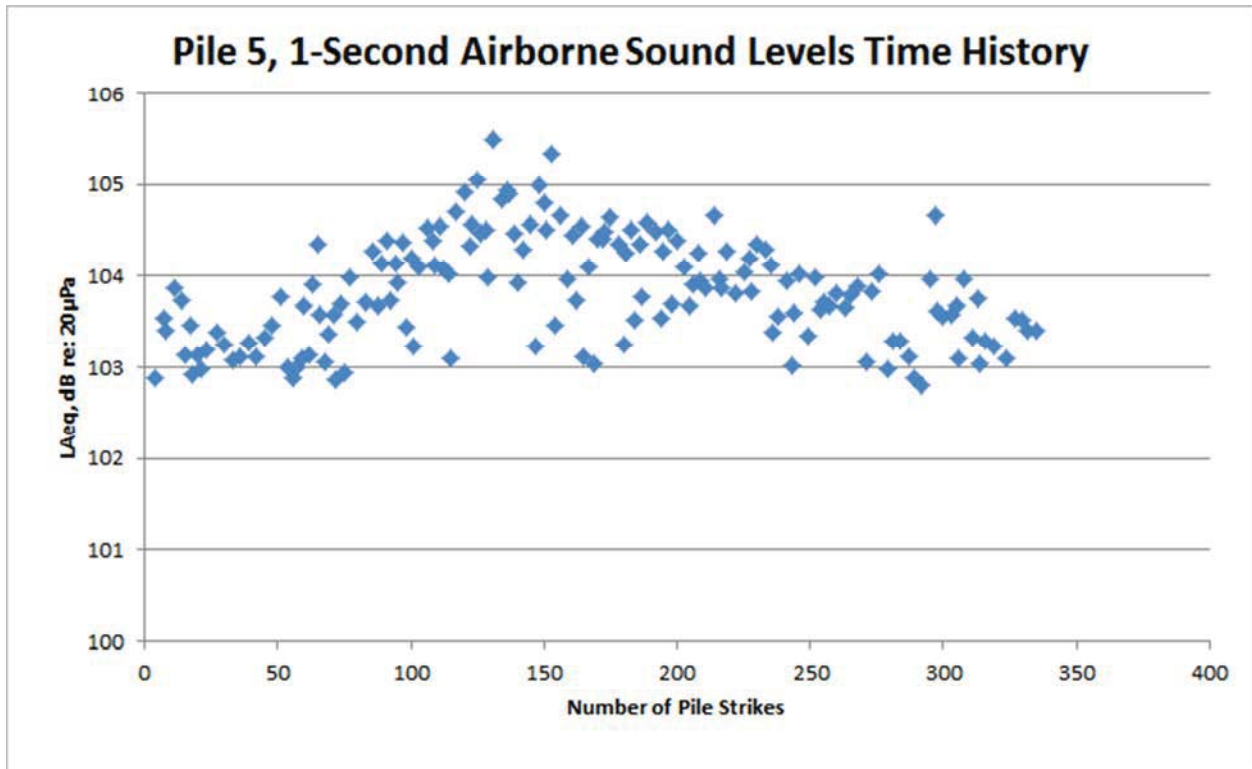
Figure 56: Pile 5, west of Foster Island airborne time history
