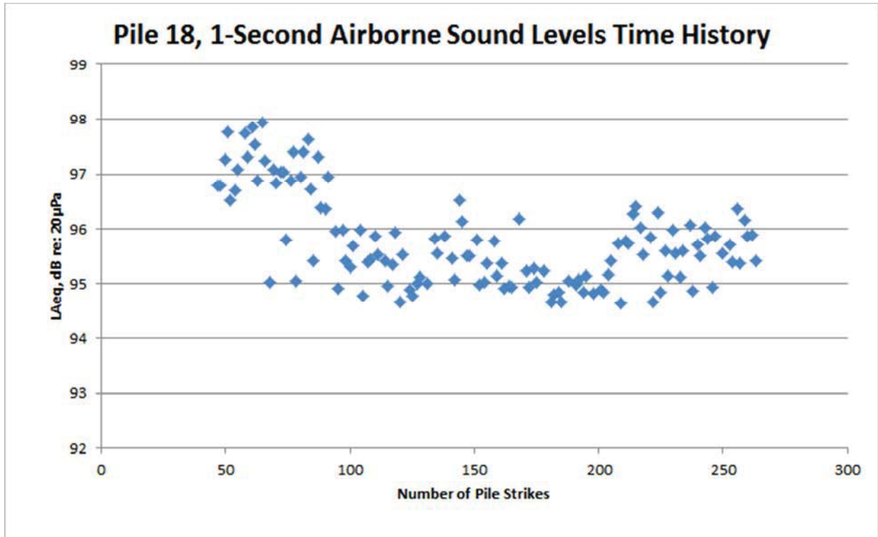
Figure 72: Pile 18, west of Foster Island airborne time history
