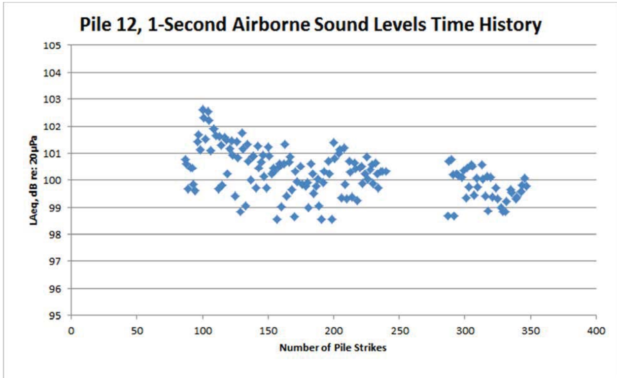
Figure 60: Pile 12, west of Foster Island airborne time history
