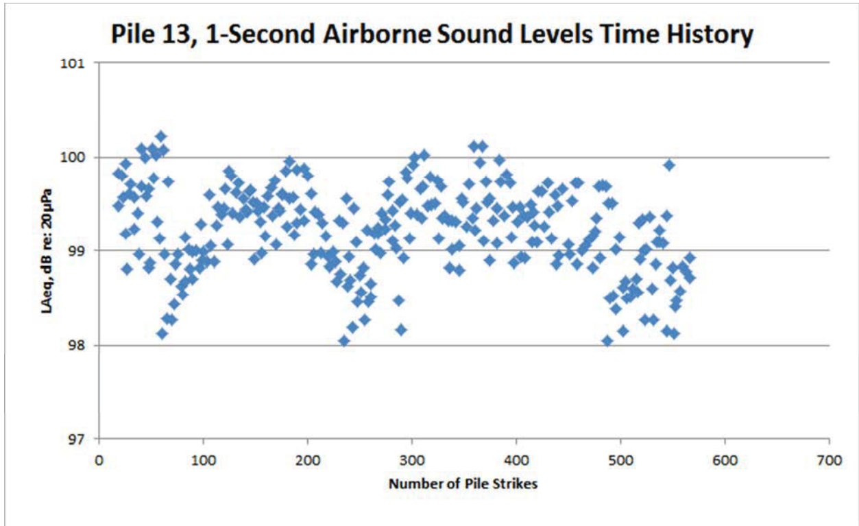
Figure 62: Pile 13, west of Foster Island airborne time history
