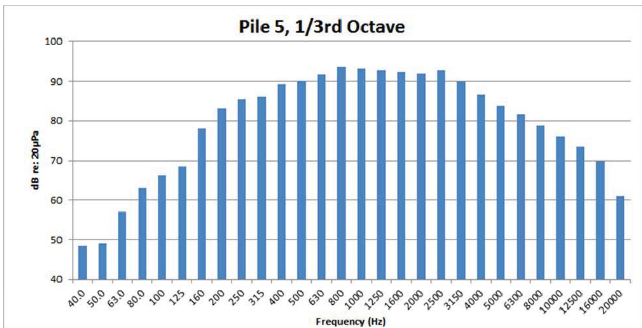
Figure 57: Pile 5, west of Foster Island airborne 1/3 rd Octave
