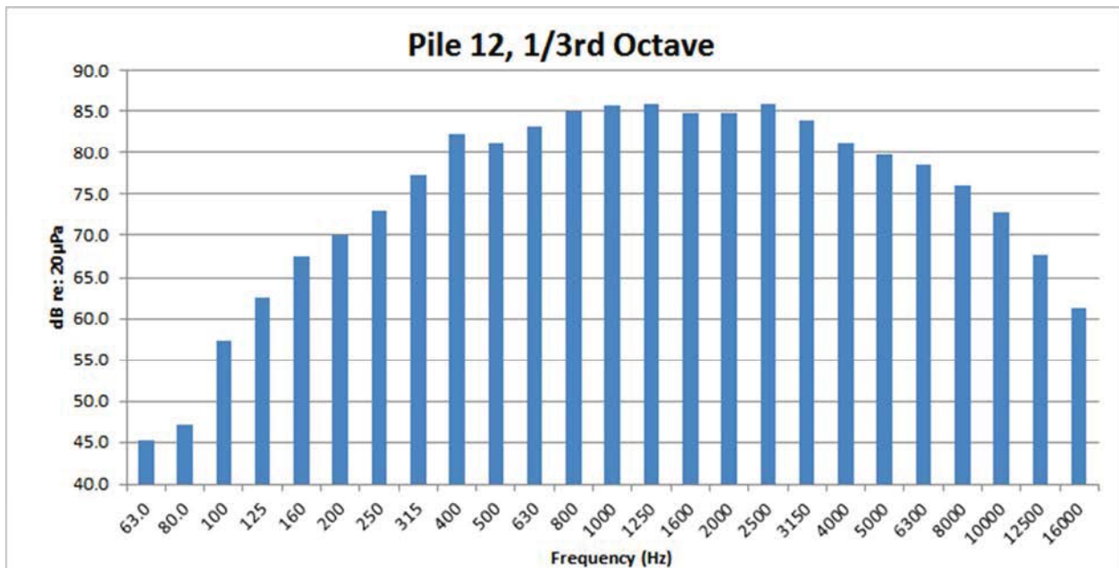
Figure 61: Pile 12, west of Foster Island airborne 1/3 rd Octave
