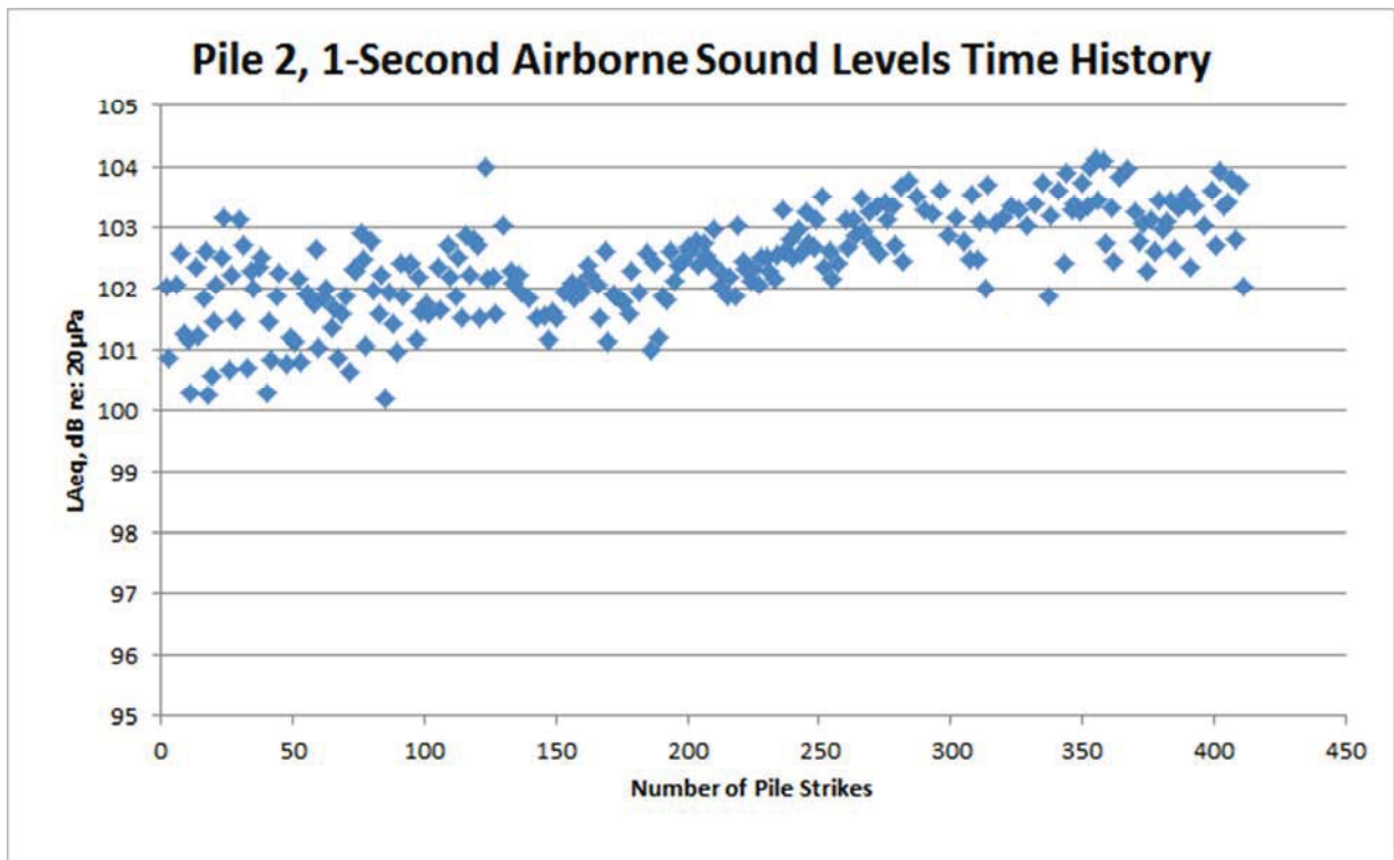
Figure 76: Pile 2, east of Foster Island airborne time history
