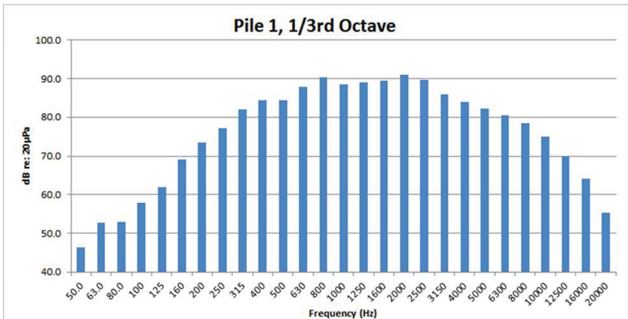
Figure 75: Pile 1, east of Foster Island airborne 1/3 rd Octave
