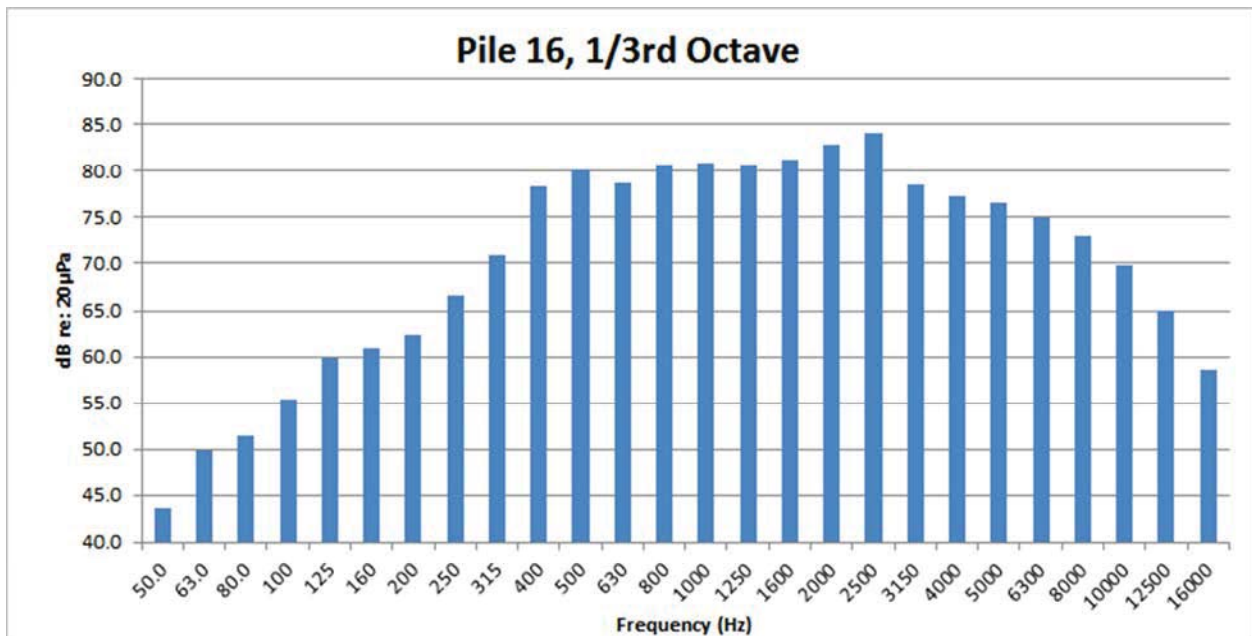
Figure 69: Pile 16, west of Foster Island airborne 1/3 rd Octave
