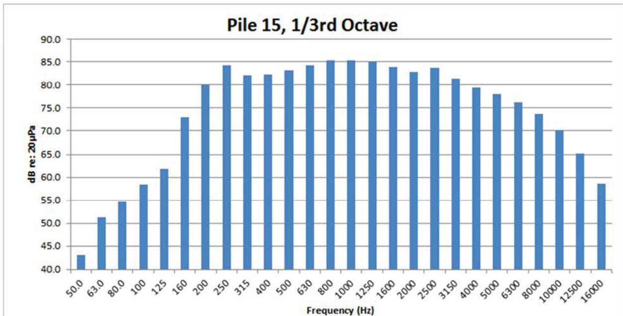
Figure 67: Pile 15, west of Foster Island airborne 1/3 rd Octave
