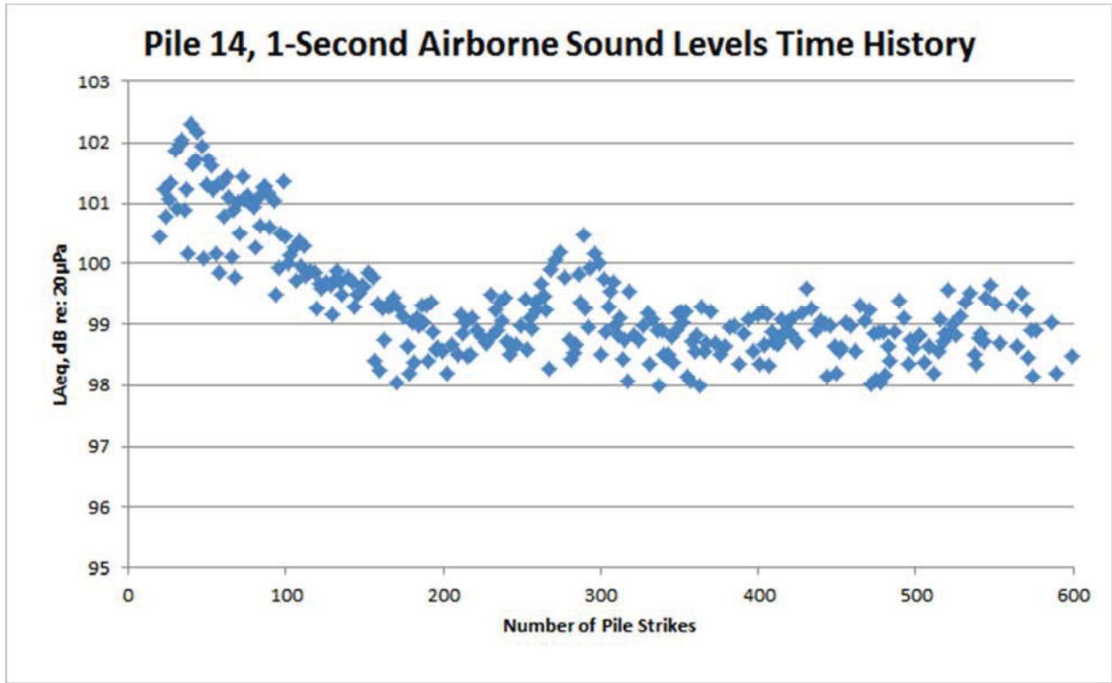
Figure 64: Pile 14, west of Foster Island airborne time history
