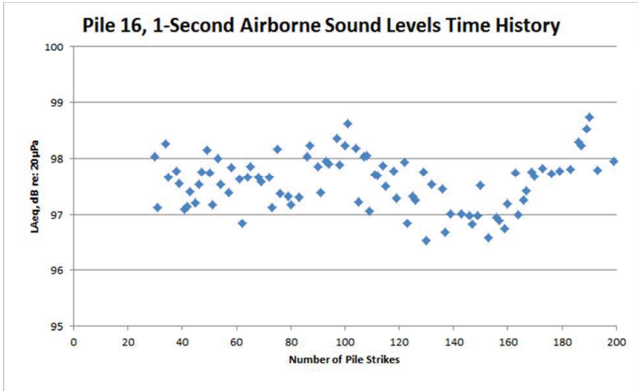
Figure 68: Pile 16, west of Foster Island airborne time history
