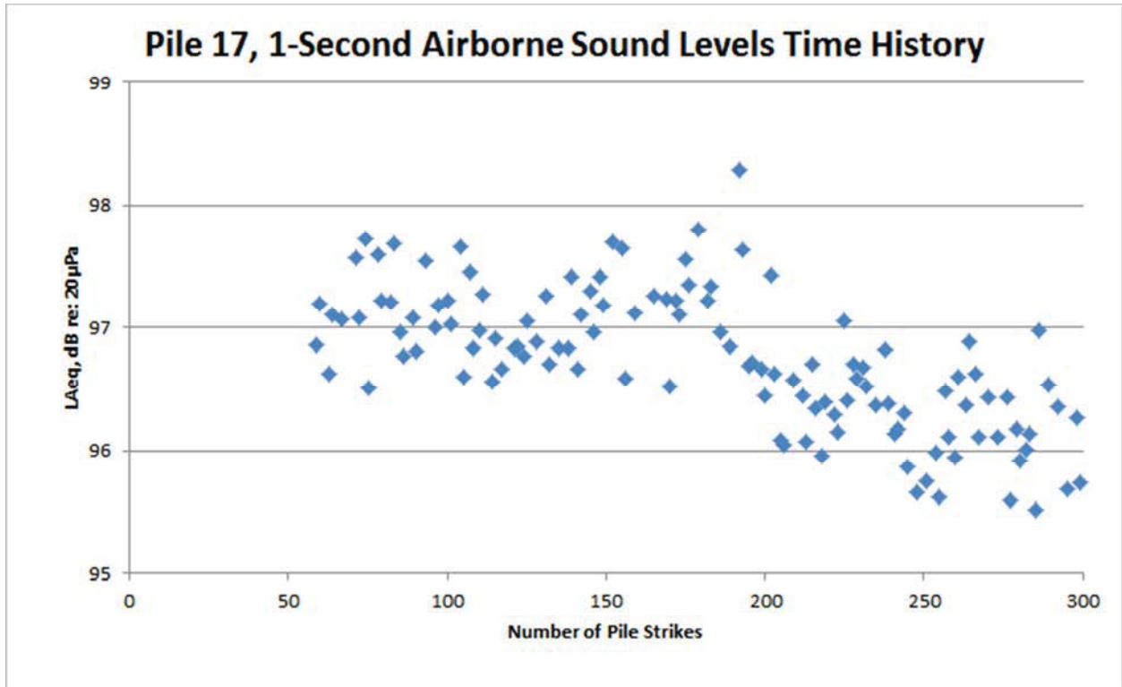
Figure 70: Pile 17, west of Foster Island airborne time history
