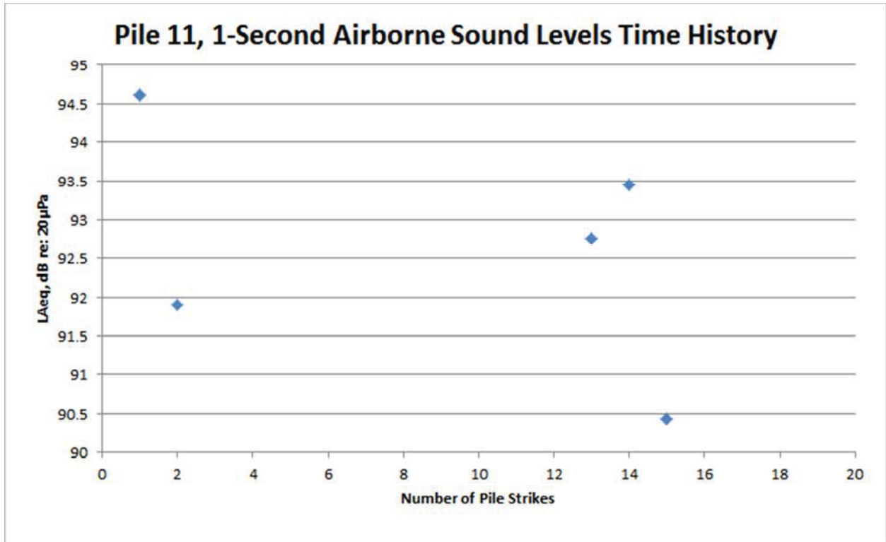
Figure 58: Pile 11, west of Foster Island airborne time history
