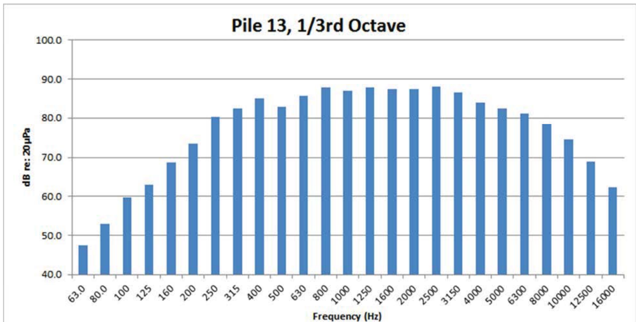
Figure 63: Pile 13, west of Foster Island airborne 1/3 rd Octave
