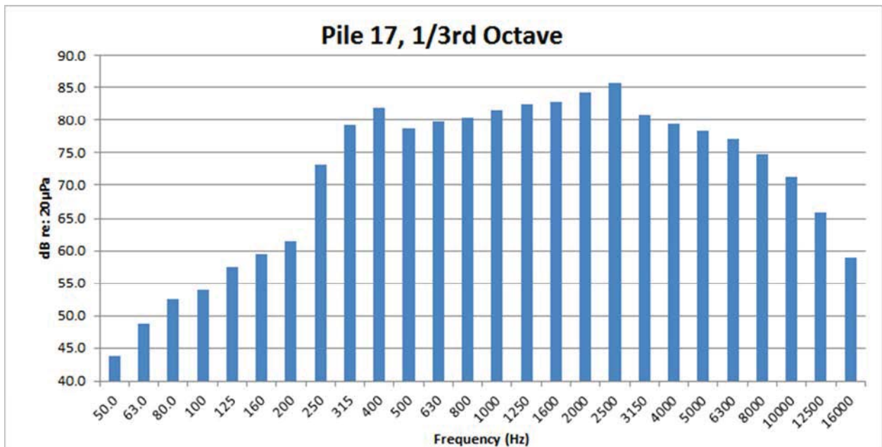
Figure 71: Pile 17, west of Foster Island airborne 1/3 rd Octave
