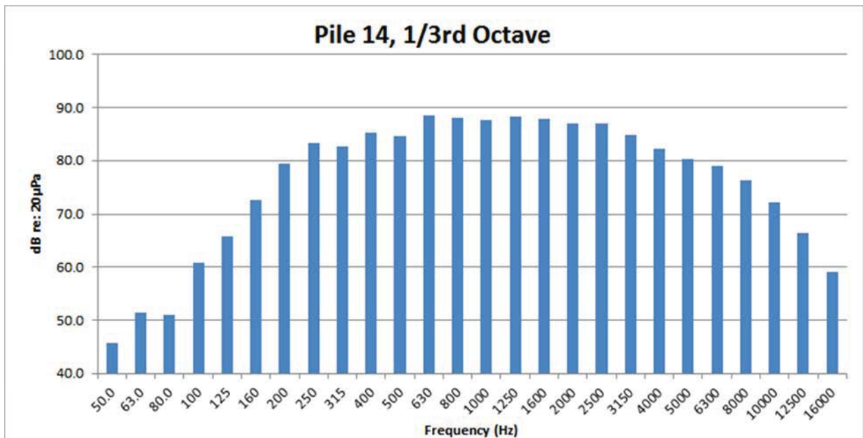
Figure 65: Pile 14, west of Foster Island airborne 1/3 rd Octave
