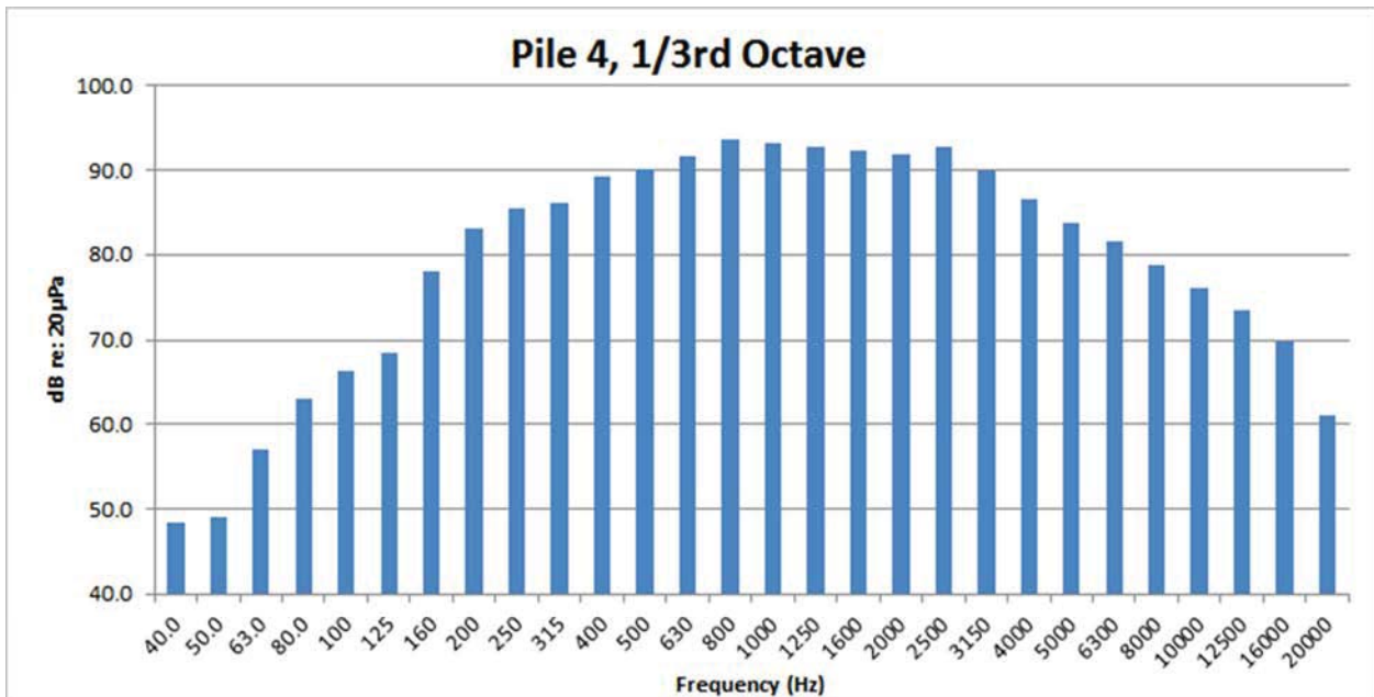
Figure 55: Pile 4, west of Foster Island airborne 1/3 rd Octave
