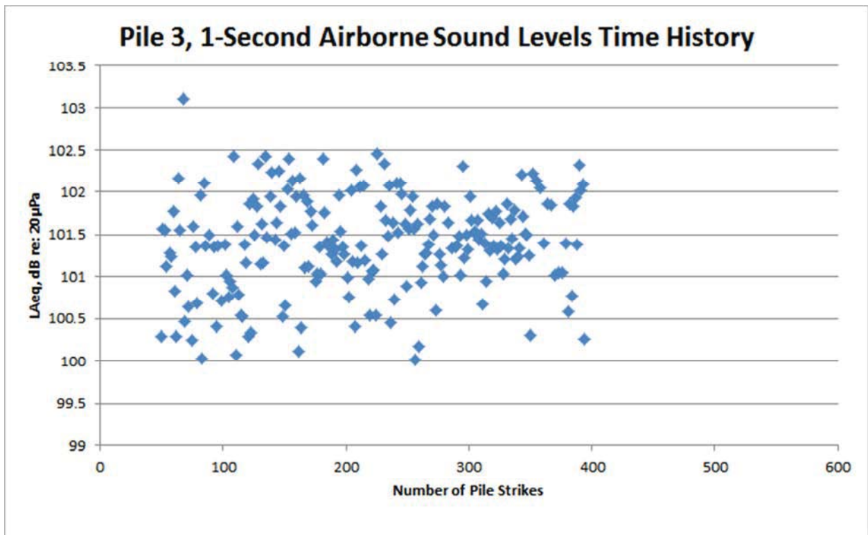
Figure 78: Pile 3, east of Foster Island airborne time history
