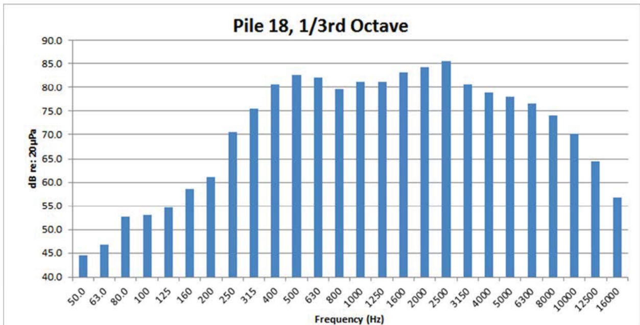
Figure 73: Pile 18, west of Foster Island airborne 1/3 rd Octave
