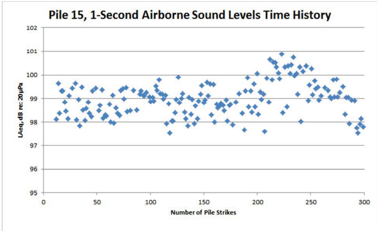
Figure 66: Pile 15, west of Foster Island airborne time history
