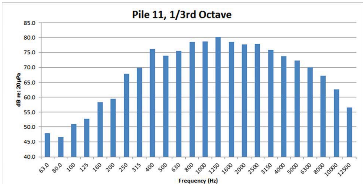
Figure 59: Pile 11, west of Foster Island airborne 1/3 rd Octave
