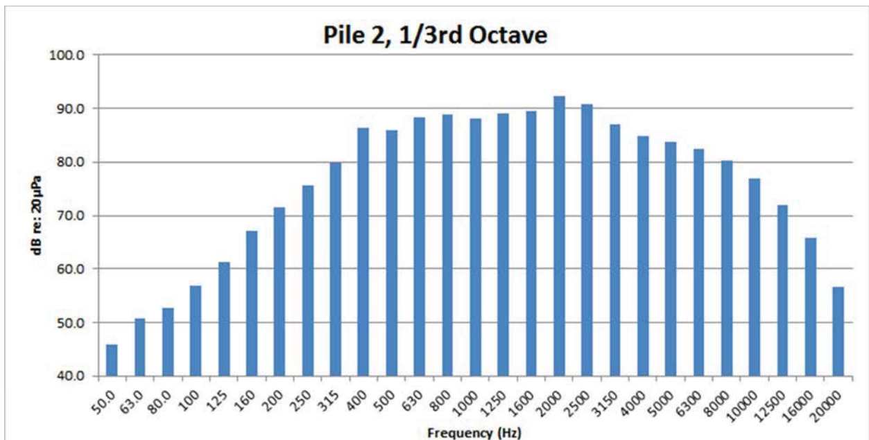
Figure 77: Pile 2, east of Foster Island airborne 1/3 rd Octave
