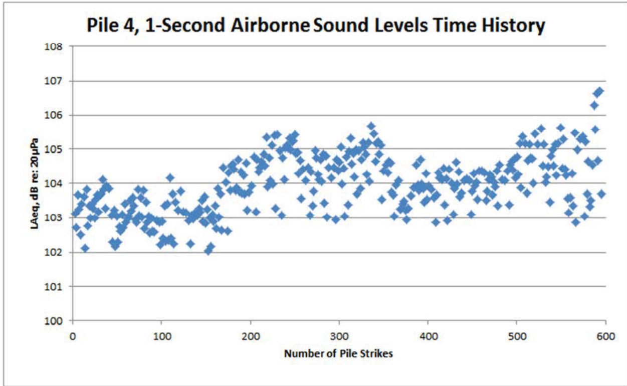
Figure 54: Pile 4, west of Foster Island airborne time history
